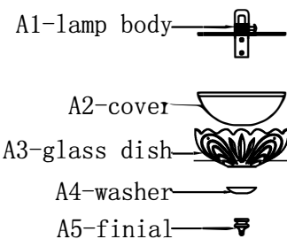
lamp body(04)parts list
